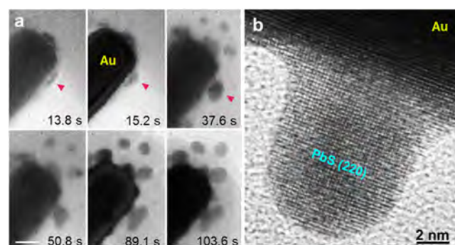
Figure 5. Effects of the CTAB surfactant on the heterogeneous growth of PbS on Au nanorods. (a) Heterogeneous nucleation and growth of PbS nanocrystals on a Au nanorod, when 150 \mu\text{L} of CTAB (0.5 M aqueous solution) is added. The red triangles indicate a PbS nanoparticle that grows into a rod shape, which is likely due to the surfactant effect. (b) HRTEM image of the as-grown single-crystal PbS nanocrystal on Au nanorod.
