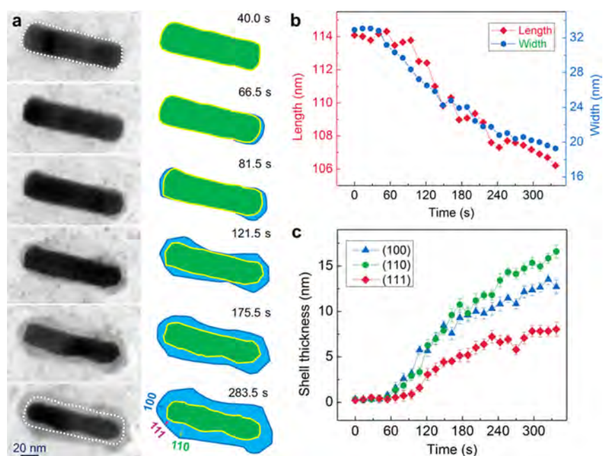
Figure 1. Heterogeneous nucleation and growth of lead sulfide on a gold nanorod. (a) TEM sequential images taken from Movie S1 and the corresponding schematic diagrams of the growth of a PbS shell on a gold nanorod. The white dashed lines on the TEM images define the contour of the original Au nanorod. (b) Length and width changes of gold nanorod during growth. (c) Dimension evolution of the shell thickness along three directions shown in (a).
