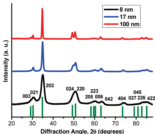
Figure 2. Powder X-ray diffraction patterns for 8, 17, and 100 nm GeTe nanocrystals. The patterns indicate the presence of phase-pure GeTe in the rhombohedral R\bar{3}m (160) space group.
