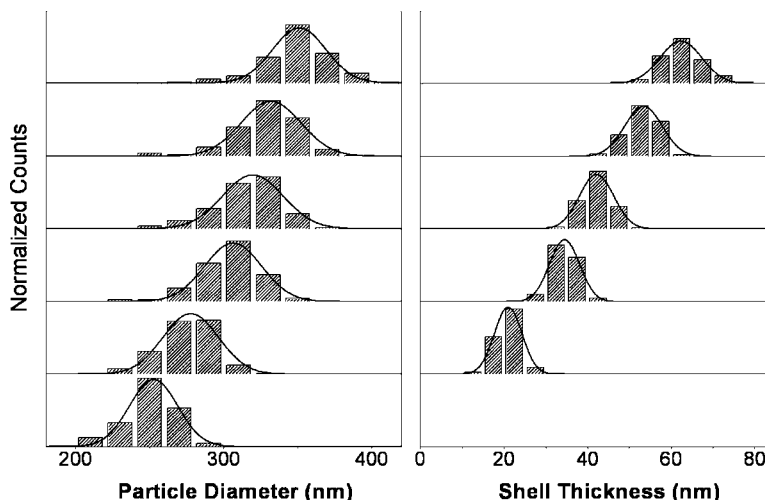
Figure 3. Particle diameter and shell thickness distributions from six aliquots at different stages of the CdS shell growth, from the initial Cd particles (bottom histograms) to the final CdS hollow particles (top histograms).
