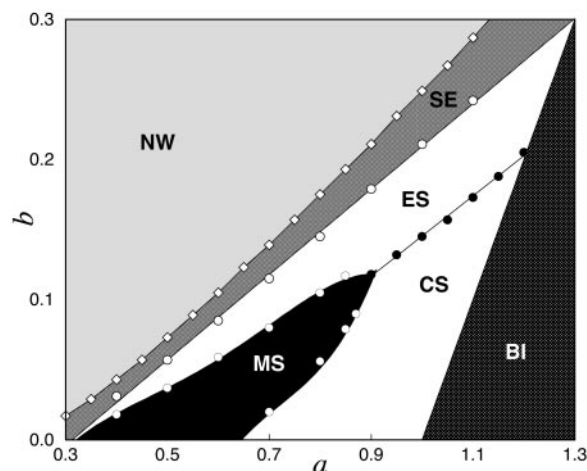
Fig. 1. Parameter space of the Barkley model. Evolution of the activator u and inhibitor v variables is governed in this model by two equations: \partial u/\partial t = \varepsilon^{-1}u(1-u)[u - (v + b)/a] and \partial v/\partial t = u - v , where \varepsilon is the ratio of the characteristic activator and inhibitor time scales, \varepsilon is fixed at 0.02 here and a and b are parameters of the model, b determining the excitation threshold. Stable 2D spiral waves are found in numerical simulations inside the entire white region, and meandering of spiral waves takes place in region MS. The 2D medium does not support excitation waves in region NW, is subexcitable (wave fragments shrink) in region SE, and is bistable in region BI. A line divides the white region into the domains where collapsing (CS) and expanding (ES) scroll rings are observed. This boundary was determined by numerical 3D simulations that assume axial symmetry of the rings. The symbols (open and solid dots and squares) indicate the points at which numerical simulations were performed. NW, no waves; SE, subexcitable; MS, meandering spirals; BI, bistable.
