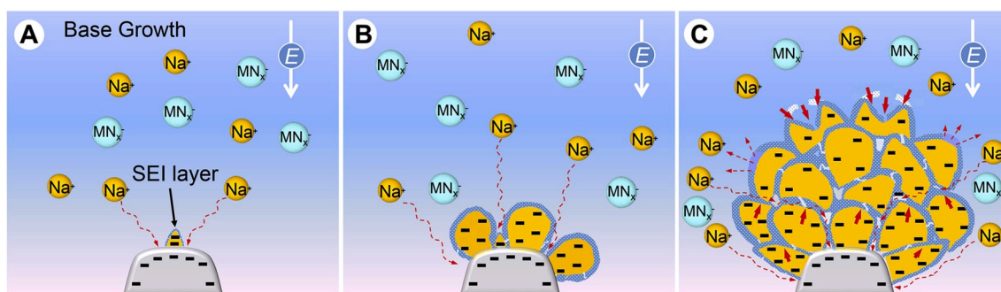
Fig. 5. Schematic illustrations of Na growth behaviors on the sharp curved electrode. (A–C) The newly formed Na grains prefer to nucleate at the base close to the electrode. The sequential deposition of Na grains and the later stage dissolution at the top of deposit are demonstrated. The SEI layer on each individual Na grain (yellow) is highlighted in blue.
