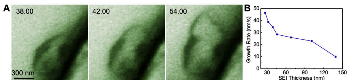
Fig. 3. Na grain growth rate versus SEI thickness. (A) Sequential images showing the growth of a Na grain. (B) Growth rate of the Na grain as a function of SEI layer thickness. The growth rate and SEI thickness were estimated at different locations of the Na grain (see more details of the measurements in Figs. S1 and S2).
