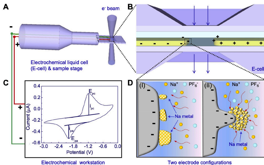
Fig. 1. A schematic of the experimental setup for in-situ TEM study of Na electrochemical deposition. (A) A custom-made electrochemical TEM sample stage. (B) An electrochemical liquid cell that fits the sample stage in (A). (C) An electrochemical program is applied to the electrochemical cell using an electrochemical workstation. (D) In-situ imaging of the electrochemical deposition of Na on the Ti electrode with different configurations composing of flat (I) or sharp (II) curvature.
