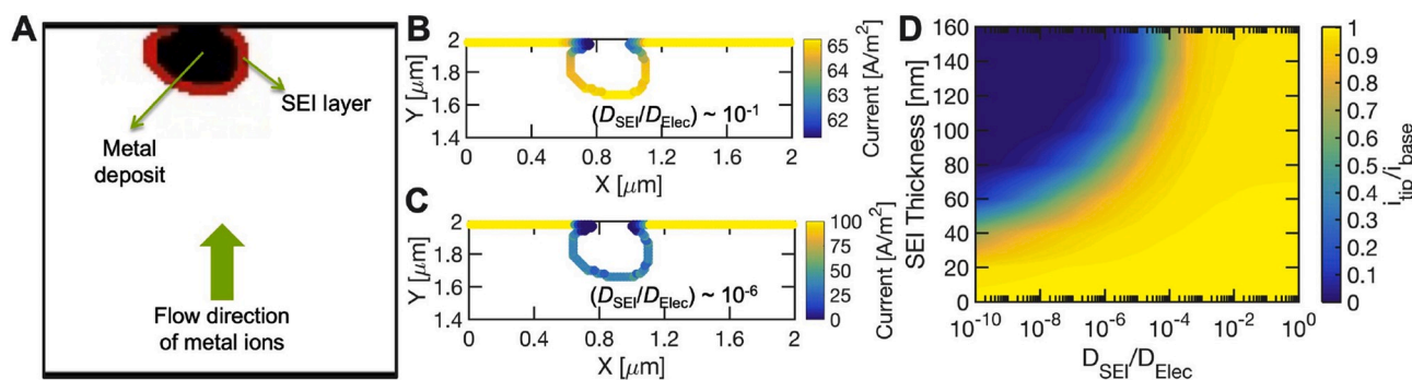
Fig. 6. Computational analysis demonstrating the SEI effects on the electrodeposition of alkali metal. (A) A schematic diagram of the computational domain adopted for the analysis. The metal deposit is denoted by the black color, and the SEI layer is depicted by red. The bottom and top electrodes (thick black lines) are 2.0\ \mu\text{m} from each other. (B) Metal deposition occurs at the tip of protrusion when metal ion transport through the SEI layer is fast. SEI diffusivity is one order of magnitude smaller than that observed in electrolyte ( D_{\text{SEI}}/D_{\text{Elec}} \sim 10^{-1} ). (C) Metal deposition is preferred at the base when ion transport through the SEI layer is slow. SEI diffusivity is six orders of magnitude smaller than that observed in liquid electrolyte ( D_{\text{SEI}}/D_{\text{Elec}} \sim 10^{-6} ). (D) A phase map between “SEI thickness” and “SEI diffusivity” (normalized as the ratio of diffusivity between SEI and electrolyte ( D_{\text{SEI}}/D_{\text{Elec}} )) demonstrates the regions where enhanced deposition should occur at the tip (yellow region), and where metal should be plated at the base (green/blue portion). For Na deposition, thickness of the SEI layer range between 100 and 140 nm, but diffusivity of Na through the SEI layer is unknown. Under the assumption of similar Na diffusivities through the SEI layer with Li ( (D_{\text{SEI}}/D_{\text{Elec}}) \sim 10^{-5} - 10^{-6} ), base growth for Na deposition is favorable.
